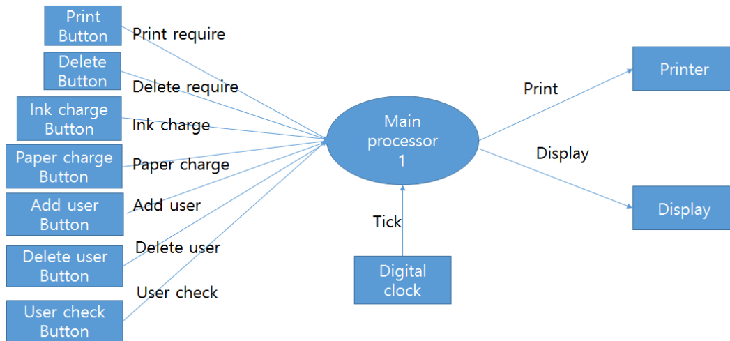
3.1.1 Basic System Context Diagram
